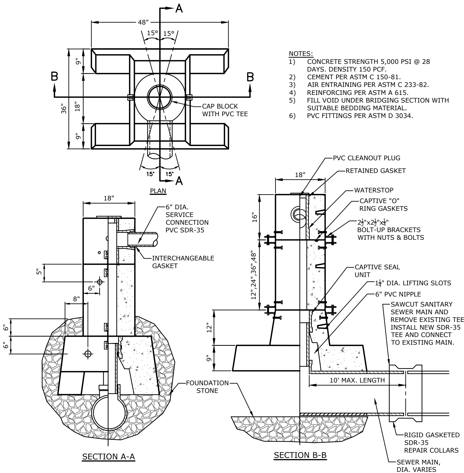
PRECAST CHIMNEY REPLACEMENT NO SCALE
