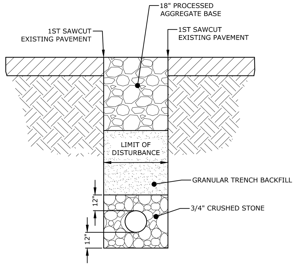
TYPICAL TRENCH DETAIL NO SCALE
