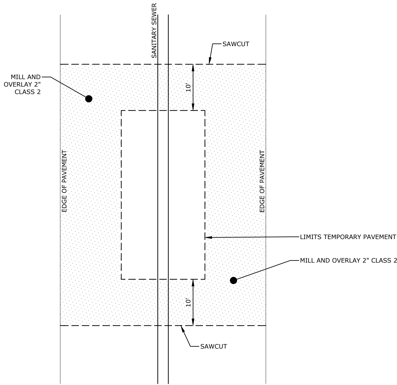
TRENCH REPAIR AREAS PERMANENT PAVEMENT REPAIR - PLAN NO SCALE
