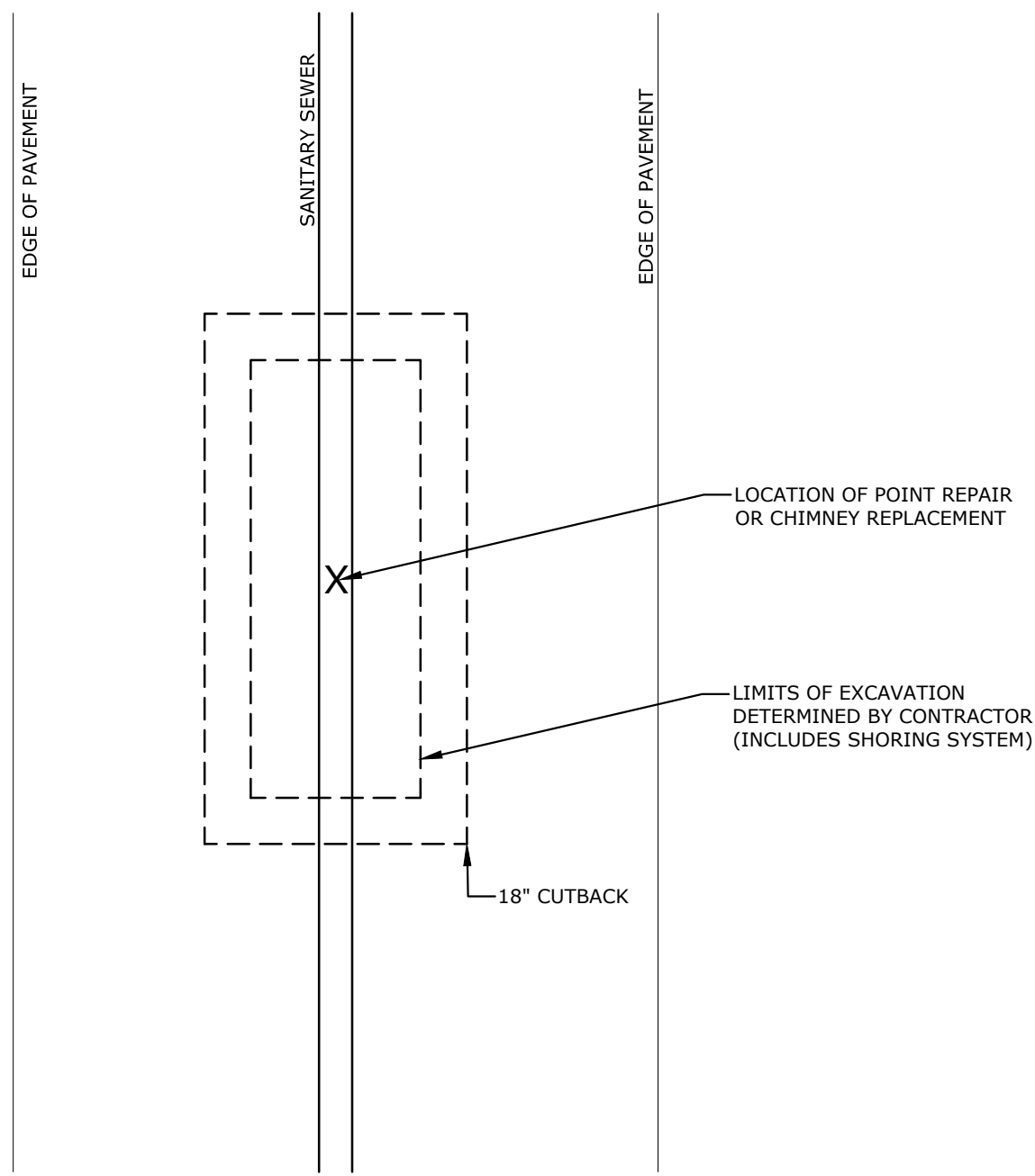
TEMPORARY PAVEMENT REPAIR - PLAN NO SCALE
