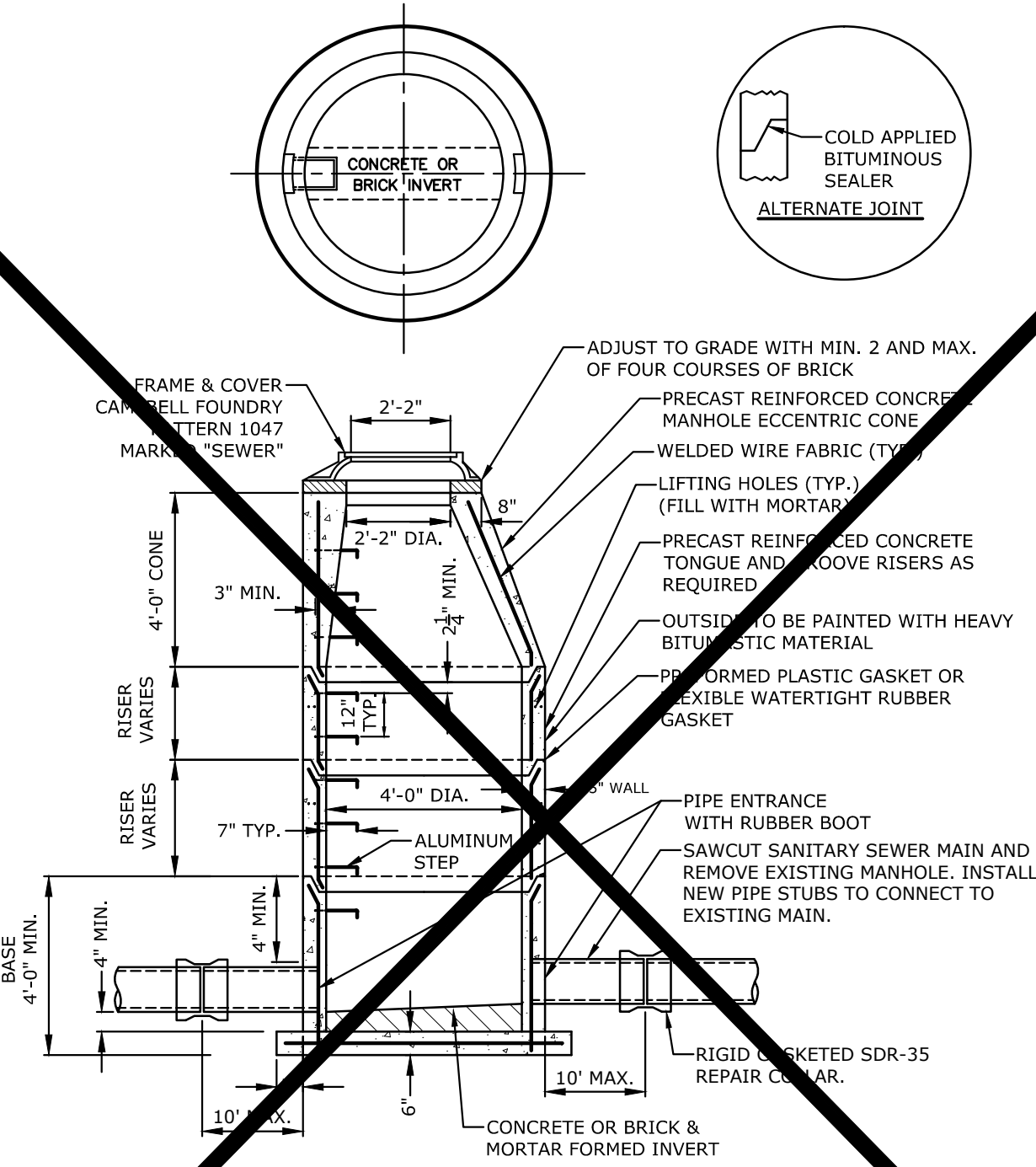
PRECAST SANITARY SEWER REPLACEMENT NO SCALE
